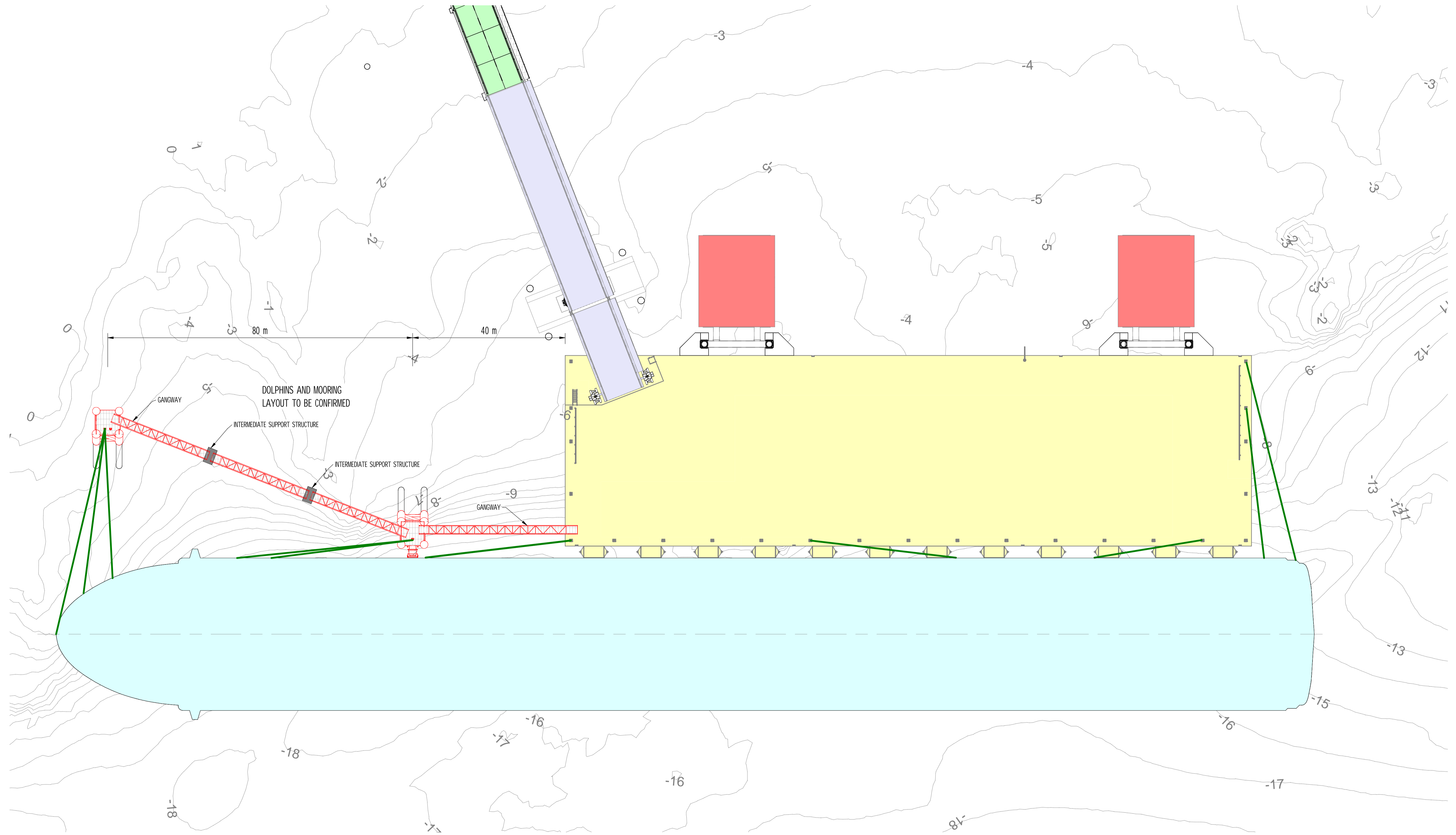
EXTENDED BERTH LAYOUT 330m VESSEL SCALE 1: 500
